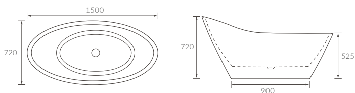
ELTERWATER FLOORSTANDING BATH
