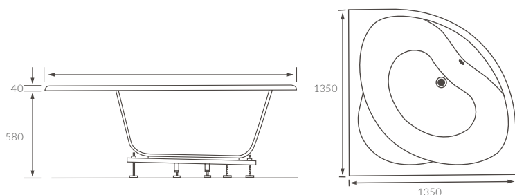
LEVEN CORNER BATH
