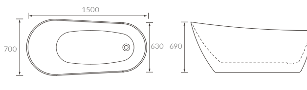
DERWENT FLOORSTANDING BATH
