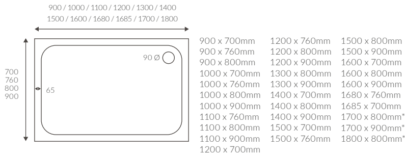
LOW PROFILE RECTANGULAR TRAYS
