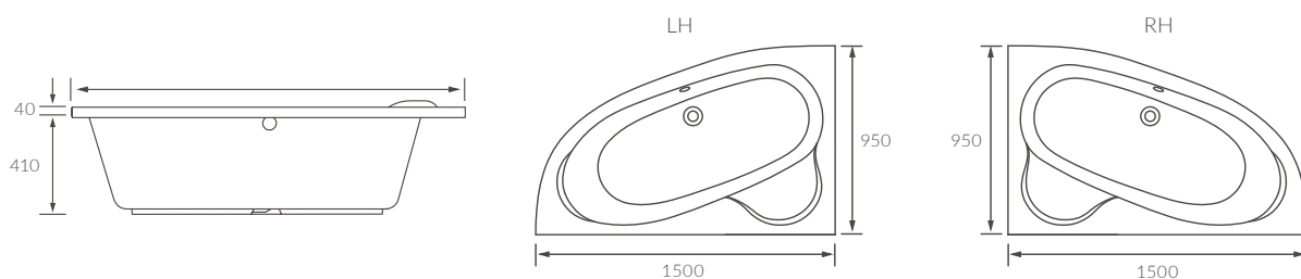
CALDEW CORNER BATH LH AND RH
