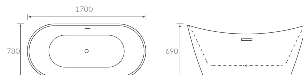
BUTTERMERE FLOORSTANDING BATH
