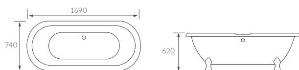
BOWSCALE DOUBLE END BATH
