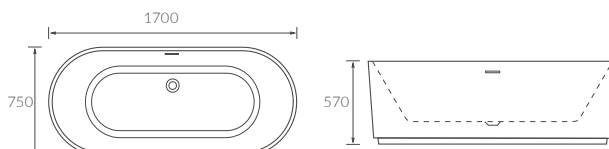
DALEHEAD FLOORSTANDING BATH
