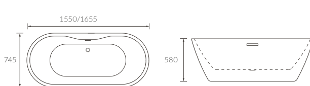
GREENDALE FLOORSTANDING BATH
