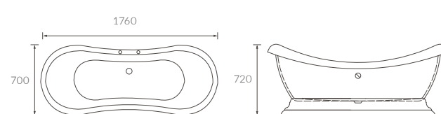
GRASMERE FLOORSTANDING BATH
