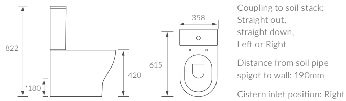
RIMLESS CLOSE COUPLED PAN AND CISTERN FULLY SHROUDED
