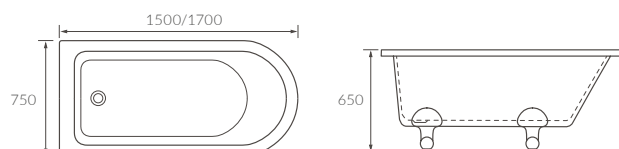
WASTWATER FLOORSTANDING BATH
